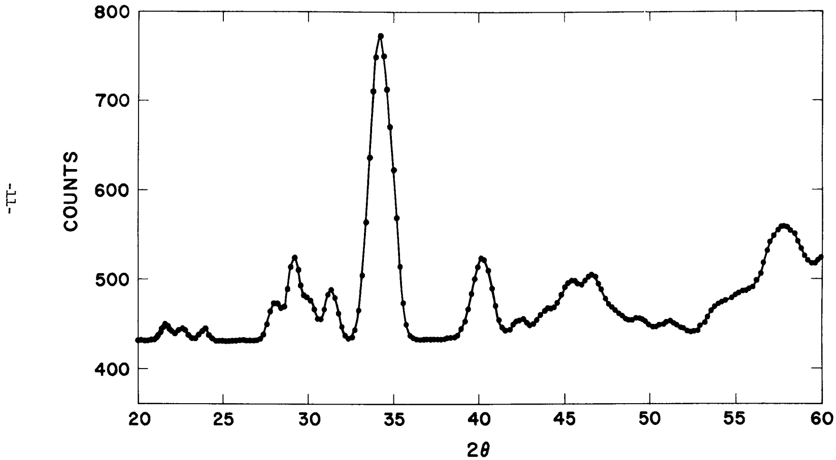
Fig. 2. Calculated neutron diffraction pattern for \alpha -Pu at 23 °K, based on Eq. (1)
